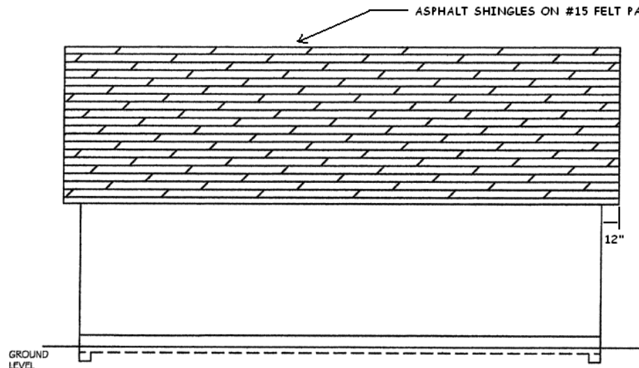
LEFT ELEVATION
